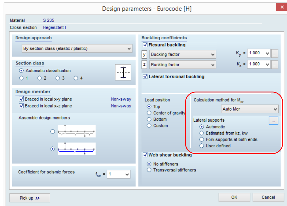
Figure 1: Design Parameters window
