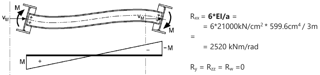
Figure 5: Possible deformation of the girder structure: non-symmetric case (source: [2])
