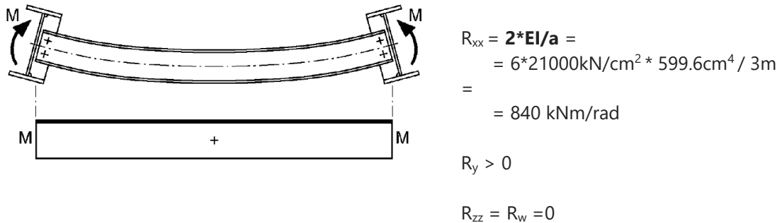
Figure 6: Possible deformation of the girder structure: symmetric case (source: [2])
